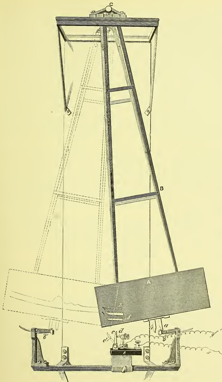
FIG. 10. THE PENDULUM MYOGRAPH.
